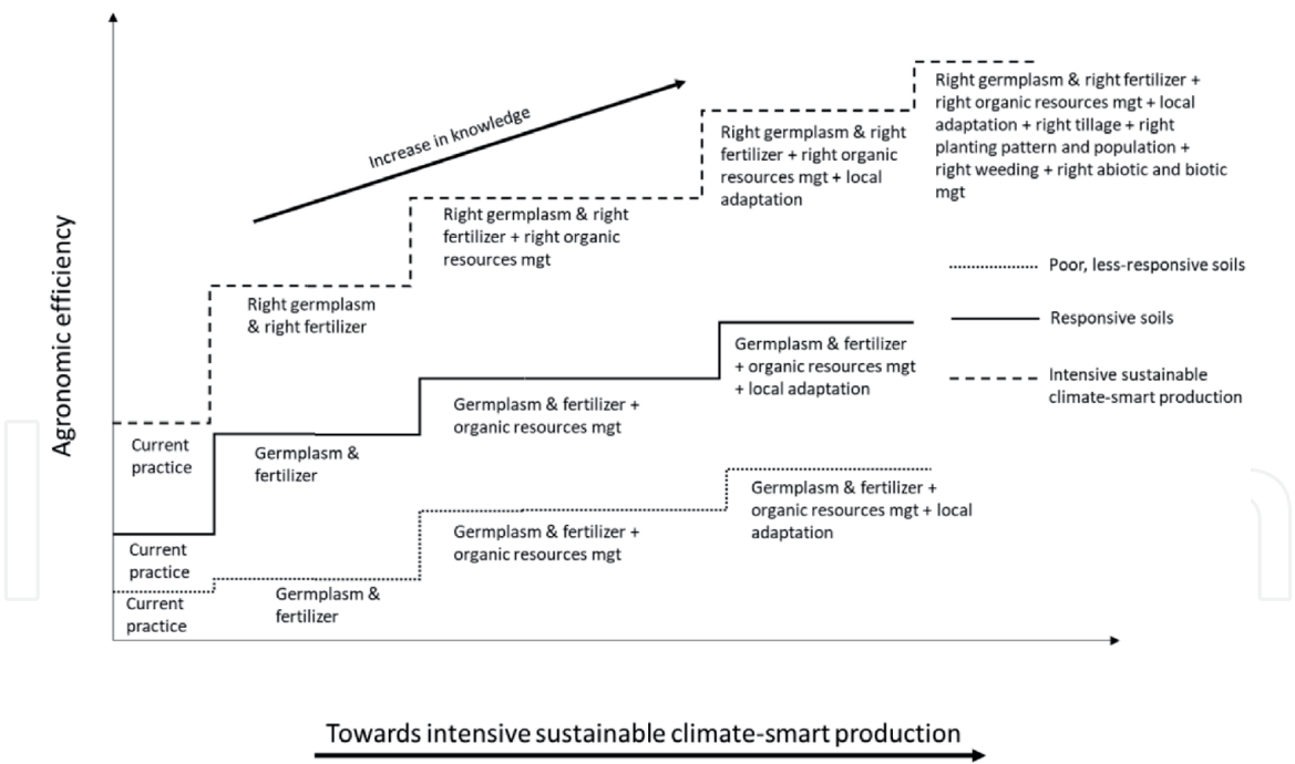
Figure 2. The components leading to intensive sustainable climate-smart production of cassava. Mgt – Management. A modified ISFM concept from [8] to achieve intensive sustainable climate-smart production.
