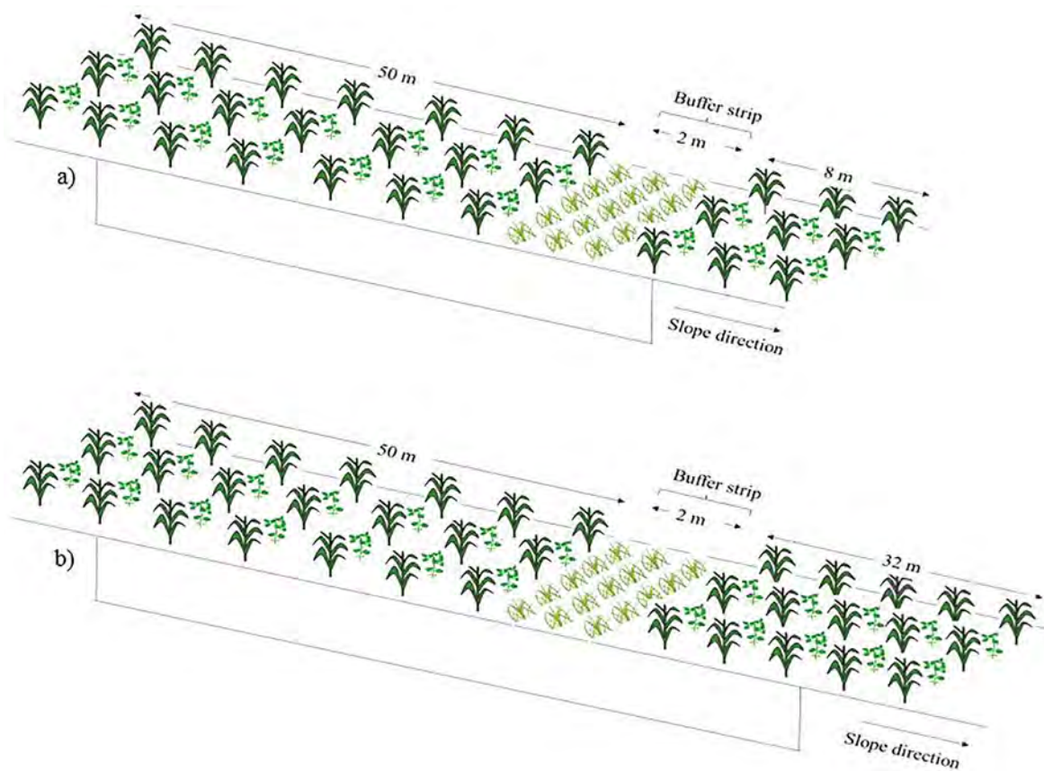
Fig. 5. Schematic diagram showing position of buffer strips at the critical slope length (50 m) on a) 60 and b) 84 m slope length.
