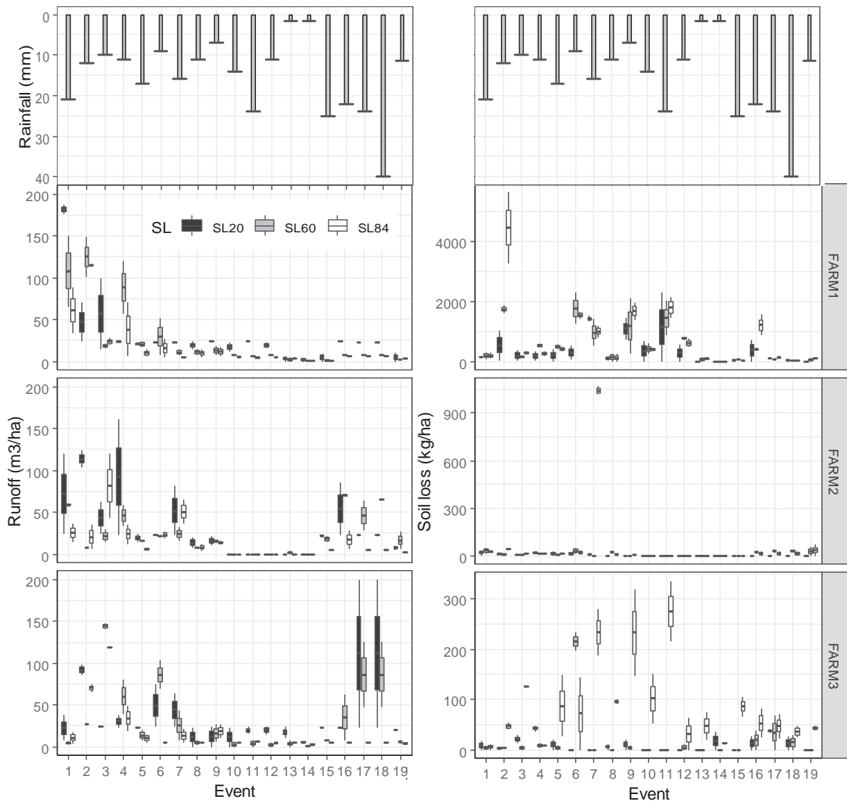
Fig. 3. Event-based runoff and soil loss under different slope lengths. Note the different y-axis scales for soil loss.
