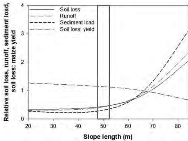
Fig. 4. Impact of slope length on soil loss, runoff, sediment load and soil-loss-to-maize-yield-ratio relative to averages across all three farms. The Vertical bar indicates critical slope length.
